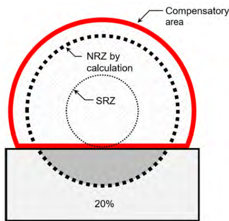
Figure 6. Sample (not to scale) of minor/moderate encroachment. AS4970:205, May 2025.
