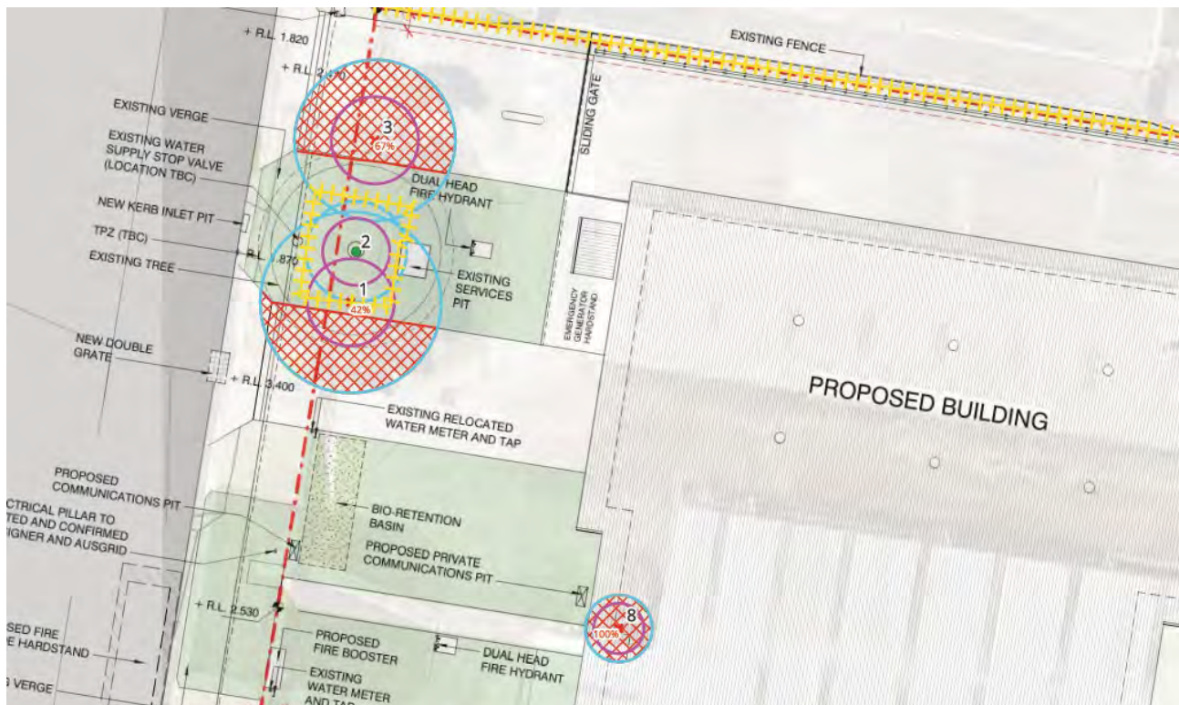
Figure 7. An image of the NRZ calculation for Tree 1, 2, 3 and 8 with the red showing the NRZ encroachment and the yellow marked line showing TPZ fencing. Appendix G - Civica ArborSafe, 2 March 2026.
